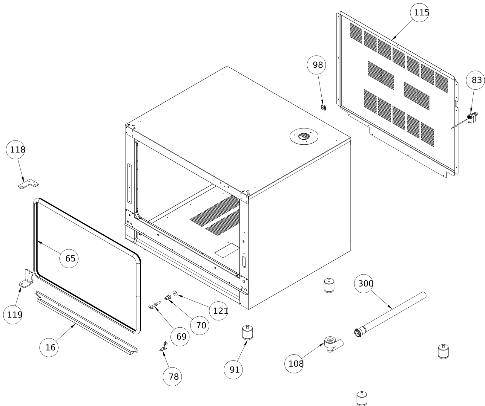
Oven body
