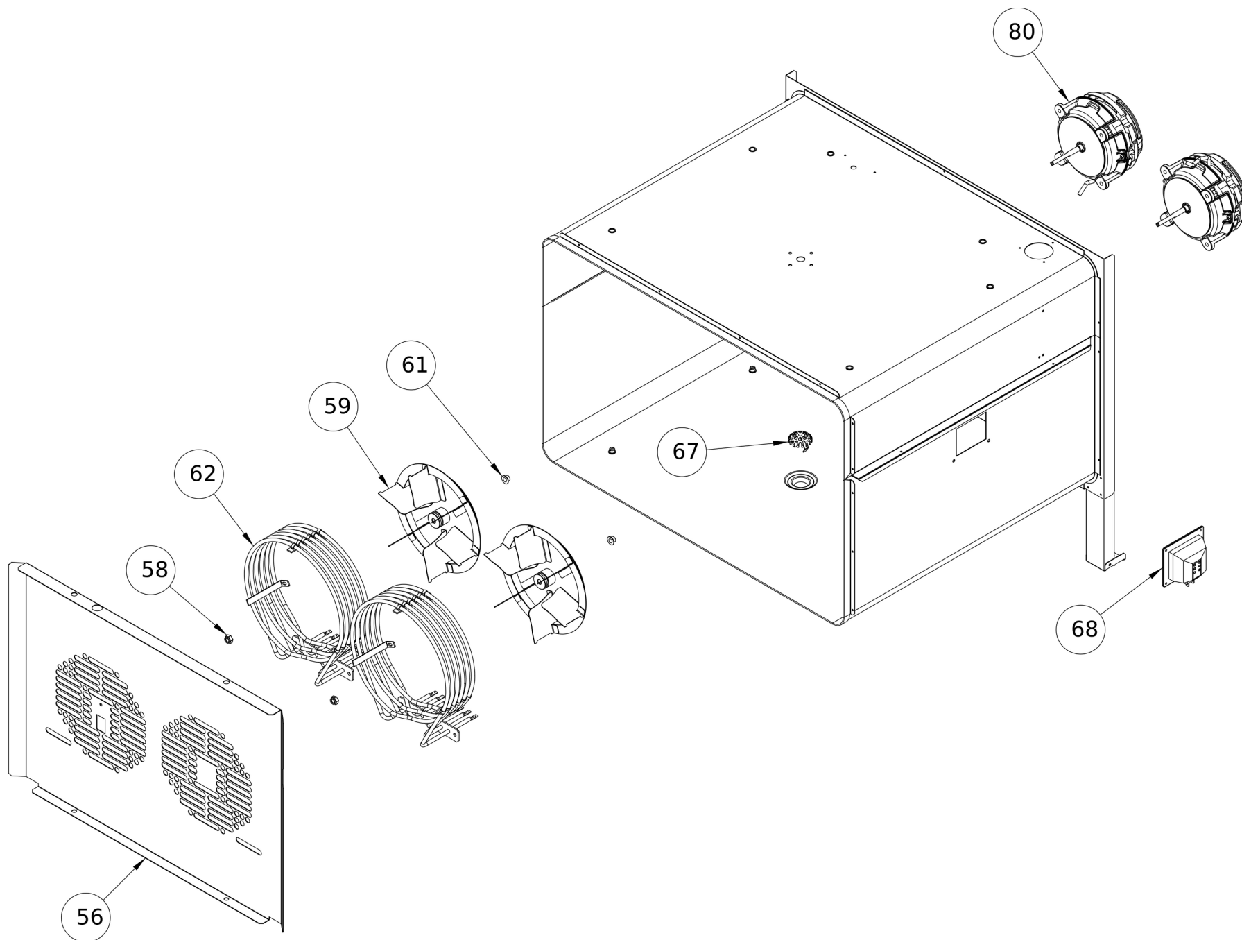
Cooking chamber
