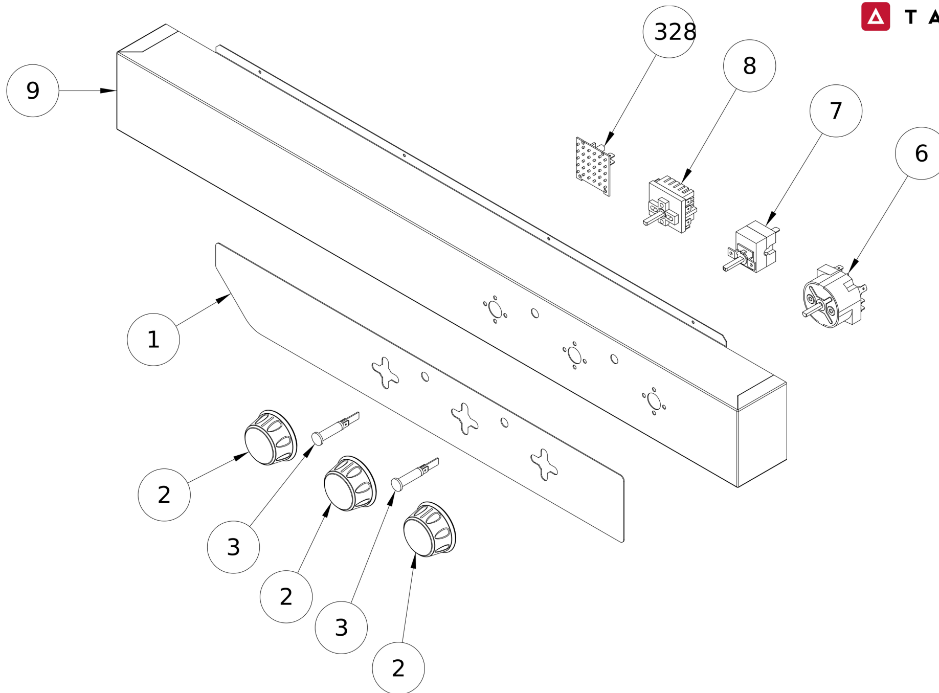
Frontal panel
